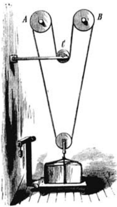
In this Scientific American illustration of Edison’s dynamometer, A is the driving pulley, B the driven pulley, and C the tension wheel; the weight to be raised and the scale are at bottom.
